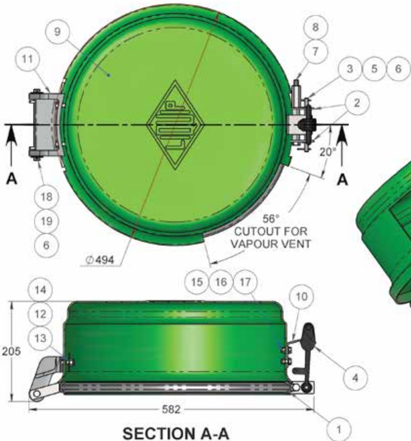
FITTED TO VOH410 HATCH
