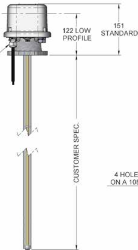
REAR VIEW
